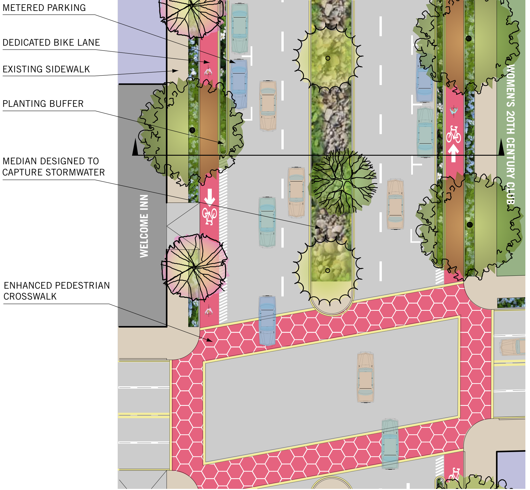
PLAN VIEW
